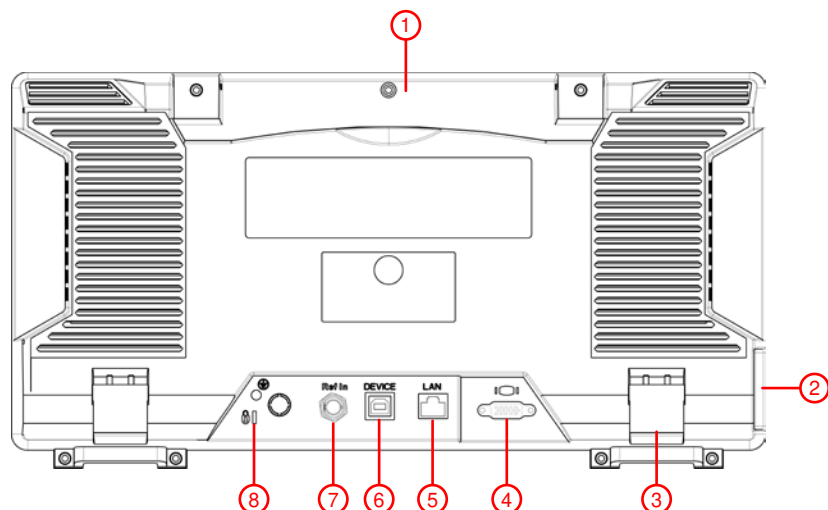
Figure 3-6 Rear Panel
